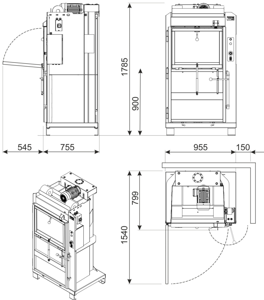
The feed door opens 90° as standard, but can be opened all the way down 180° for customized needs.
